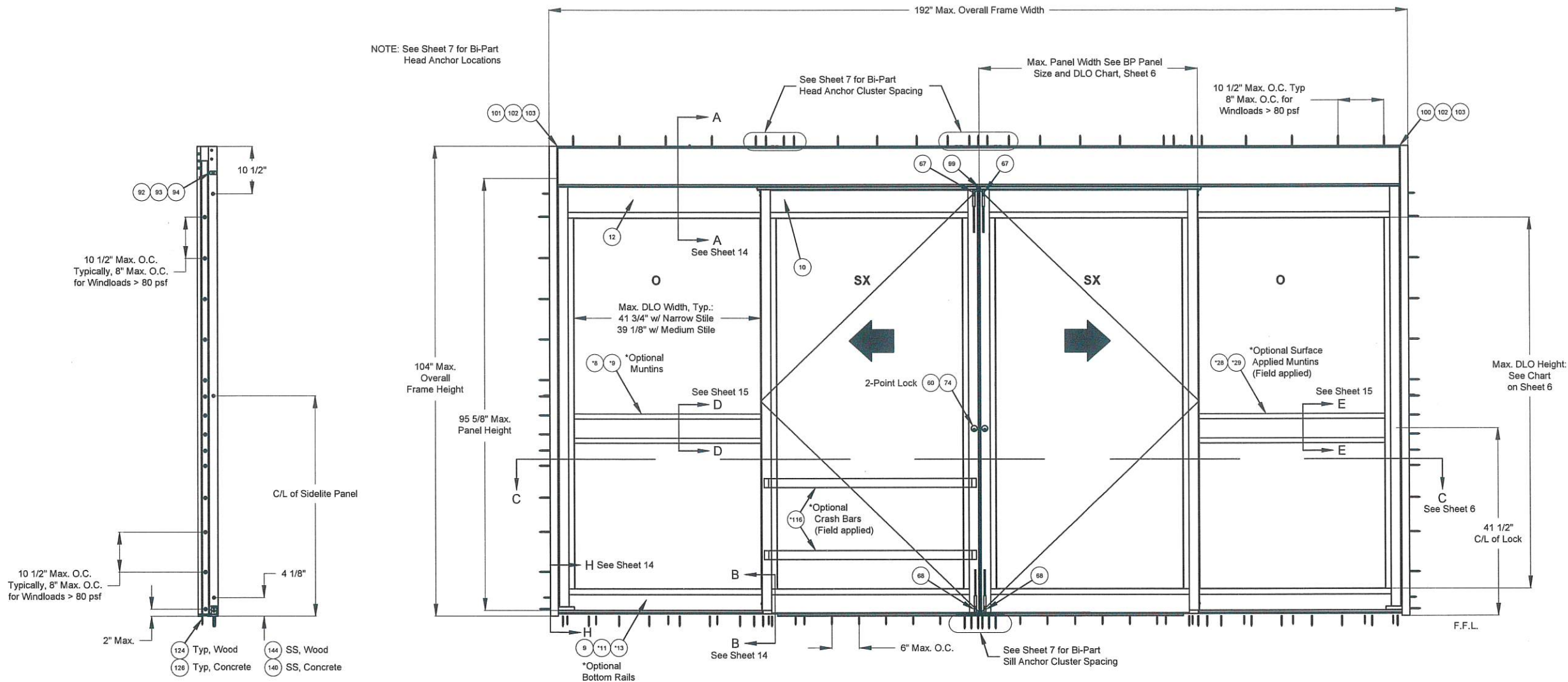
BP FSL (4 PANELS, BI-PART FIXED SIDELITE)
